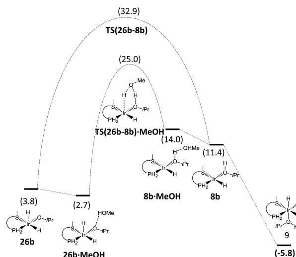
Figure 6. Alternative O–H coupling/ \text{H}_2 oxidative addition pathway for the regeneration of the resting state 9 from 26b .
