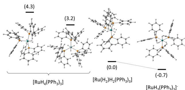
Figure 3. Relative energy in methanol solution ( \Delta G_{\text{MeOH}} in kilocalories per mole) of three “ \text{RuH}_4(\text{PPh}_3)_3 ” isomers and of the deprotonated complex [\text{RuH}_3(\text{PPh}_3)_3]^- .
