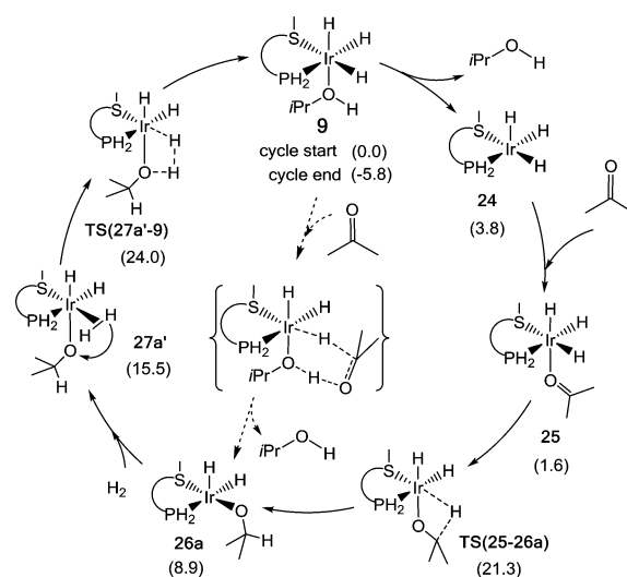
Figure 5. Best cycle for acetone hydrogenation catalyzed by [\text{IrH}_4(1^{\text{Ph}})(i\text{PrOH})] (9). For each species the Gibbs energy in kcal/mol is given in parentheses below the compound symbol.
