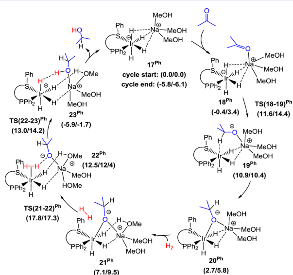
Figure 4. Computed cycle for acetone hydrogenation catalyzed by [\text{Na}(\text{MeOH})_3][\text{IrH}_4(1^{\text{Ph}})] ( 17^{\text{Ph}} ). For each species the Gibbs energies (optimized geometry with BS1/ fixed geometry with BS2) in kilocalories per mole are given in parentheses below the compound symbol.
