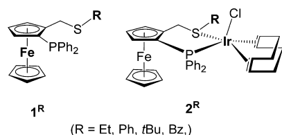
Scheme 2. Ligand and Precatalyst Object of This Study
