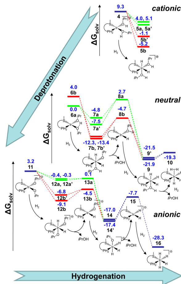
Figure 1. Relative energy in methanol solution ( \Delta G_{\text{MeOH}} in kilocalories per mole) of various species generated from [\text{Ir}(\text{COD})-(\text{PS})]^+/\text{H}_2/[\text{MeO}(\text{MeOH})_5]^- . Only the structures of the lowest energy isomers are shown. See the SI for the others. Color coding: green, (a isomers, H trans to P); red (b isomers, H trans to S); blue (numbers with no letter, primed numbers for isomers), symmetric systems.
